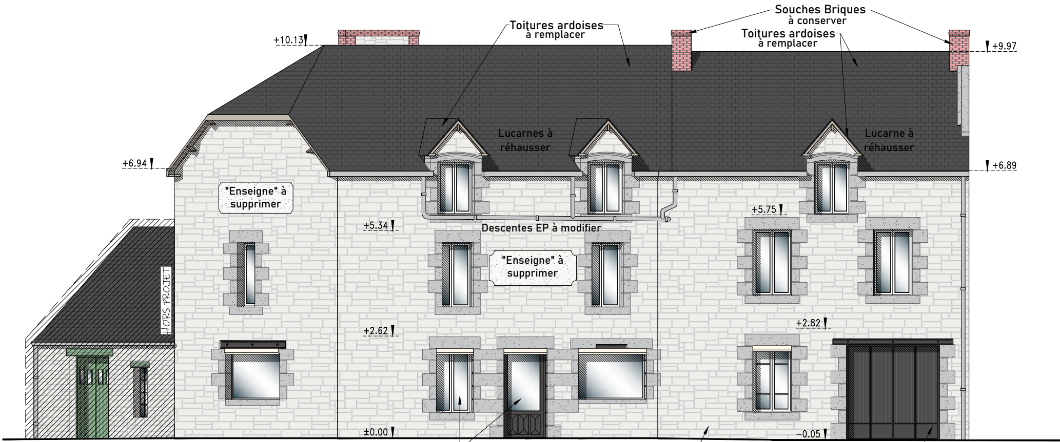
FACADE SUD
